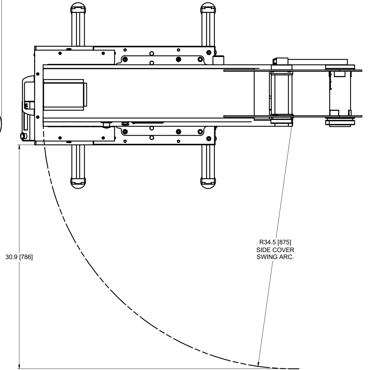
VIEW C-C
